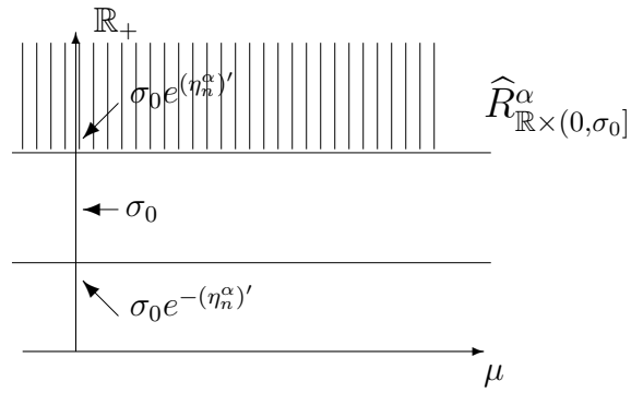
Figure 6.8: Rejection region \hat{R}_{\mathbb{R} \times (0, \sigma_0]}^\alpha
