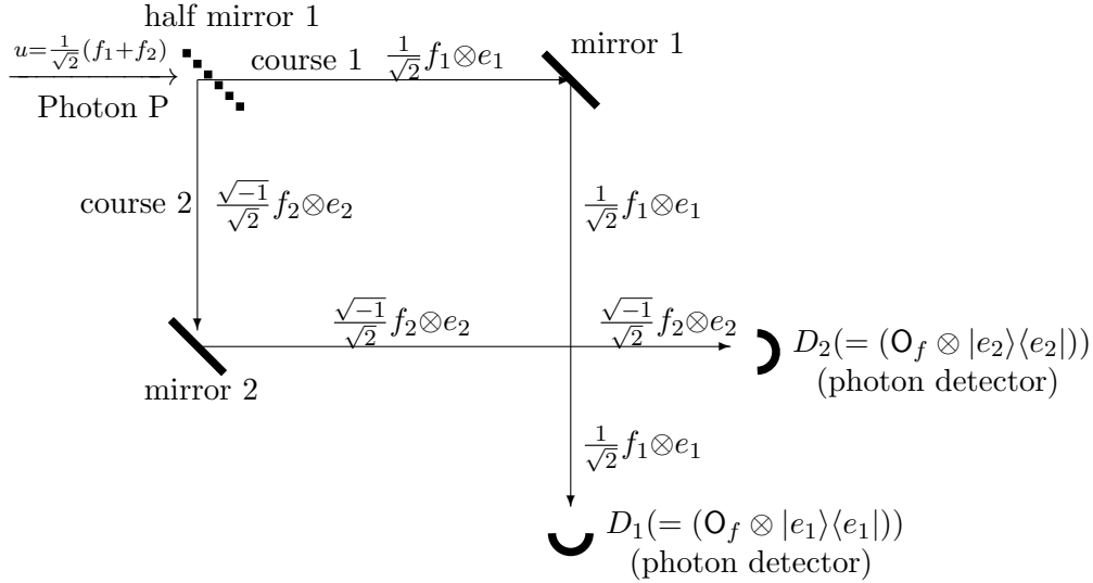
Figure 11.4(1'). [D_1 + D_2] = O_f \otimes O_E
