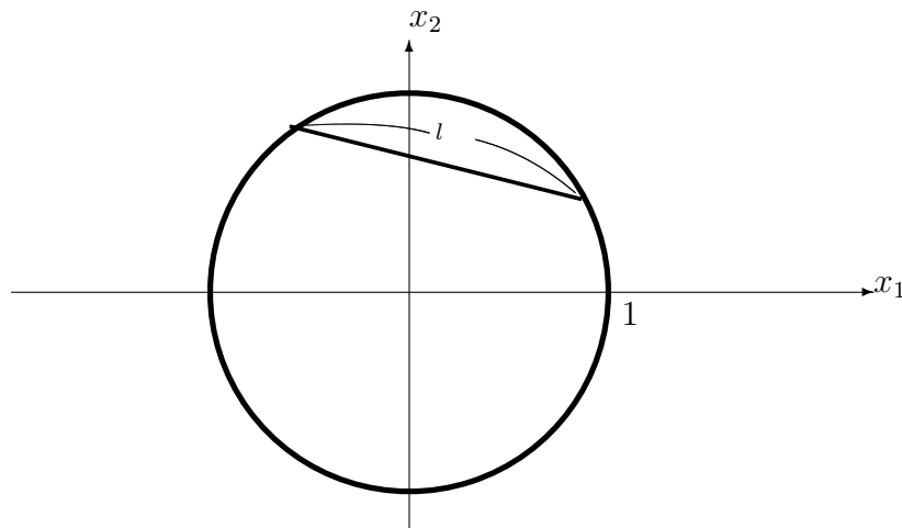
Figure 9.9: Bertrand's paradox
