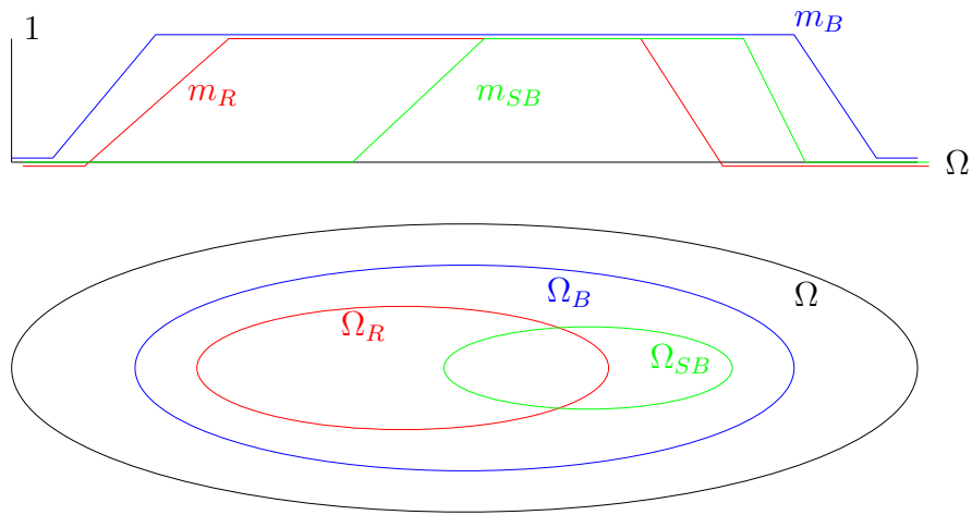
Figure 20.4: [All ravens are black: ( \Omega_R \subseteq \Omega_B ) ]
