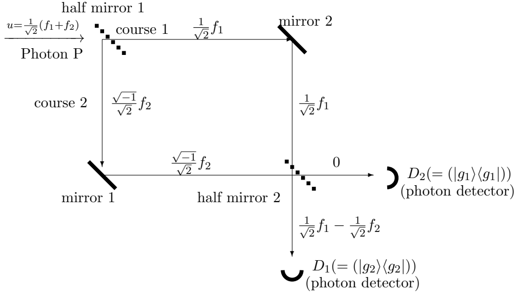
Figure 11.4(2). [D_1 + D_2] = \text{Observable } O_g
