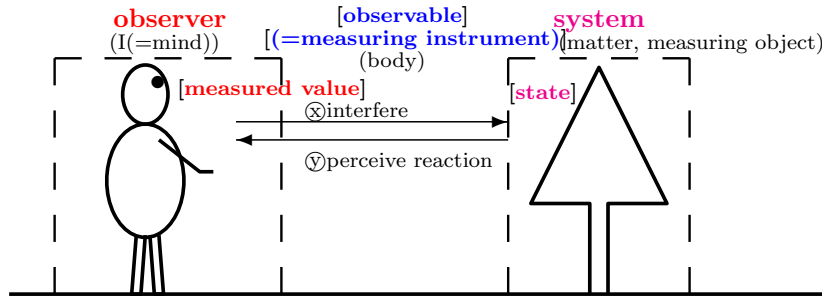
Figure 10.1: (=Figure 3.1)[Descartes Figure]: Image of “measurement(= \otimes + \otimes )” in mind-matter dualism
