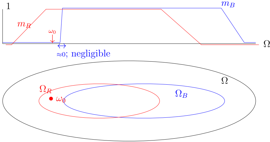
Figure 20.3: [\omega_0 \in \Omega_R \setminus \{\omega \mid m_B(\omega) = 0\}, \rho_0(\{\omega \in \Omega \mid 0 < m_B(\omega) < 1\} \cap \Omega_R)] \approx 0 , i.e., negligible. ]
