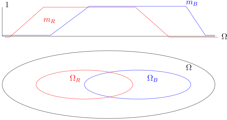
Figure 20.1: [Raven state class \Omega_R , black bird state class \Omega_B ]
