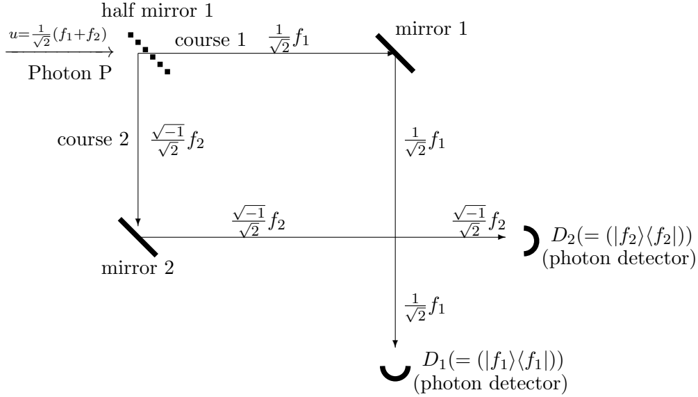
Figure 11.4(1). [D_1 + D_2] = \text{Observable } O_f
