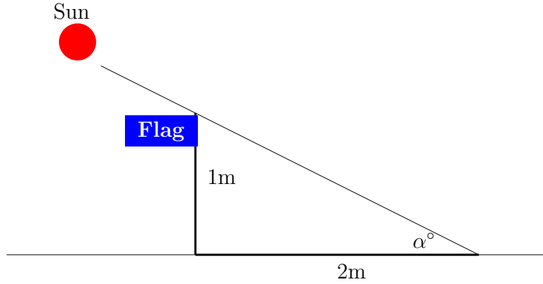
Figure 12.5: [Flagpole problem ]
