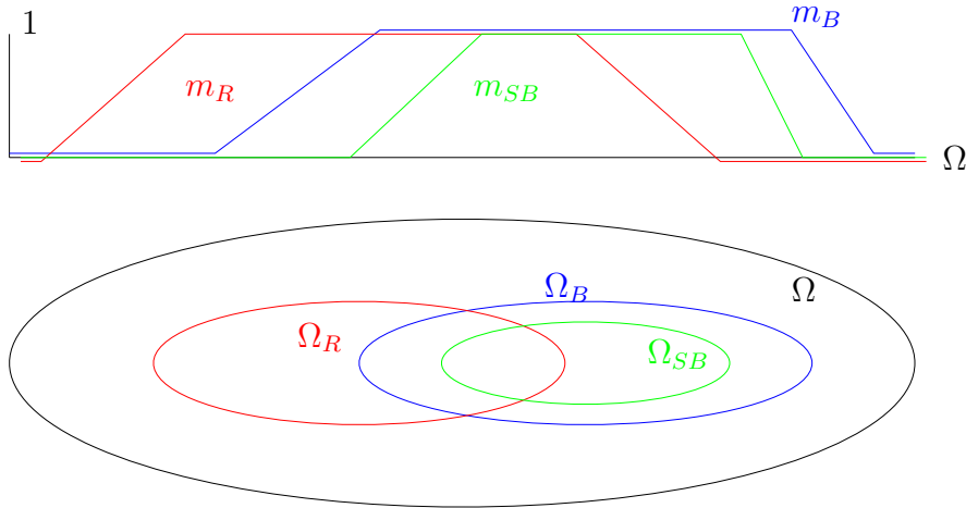
Figure 20.2: [Raven state class \Omega_R , black bird state class \Omega_B , small black bird state class \Omega_{SB} ]
