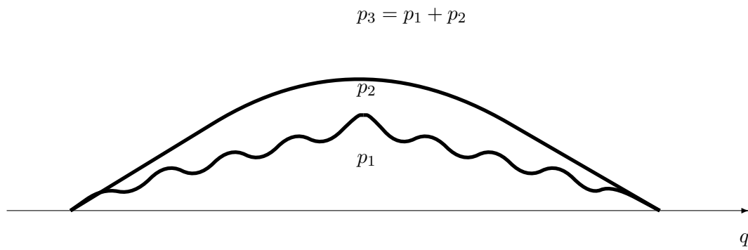
Figure 11.6(3): The graph of p_3 = p_1 + p_2
