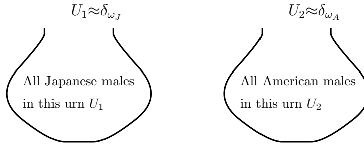
Figure 5.1: Population ≈ urn (↔ state)
