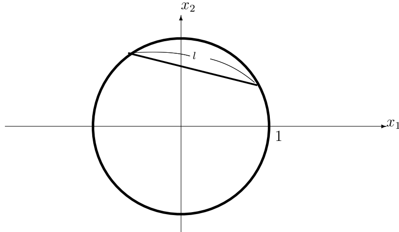
Figure 9.8: Bertrand's paradox
