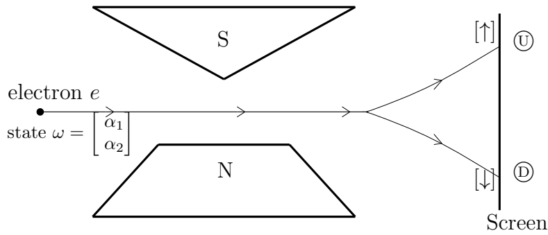
Figure 2.10: Stern–Gerlach experiment (1922)
