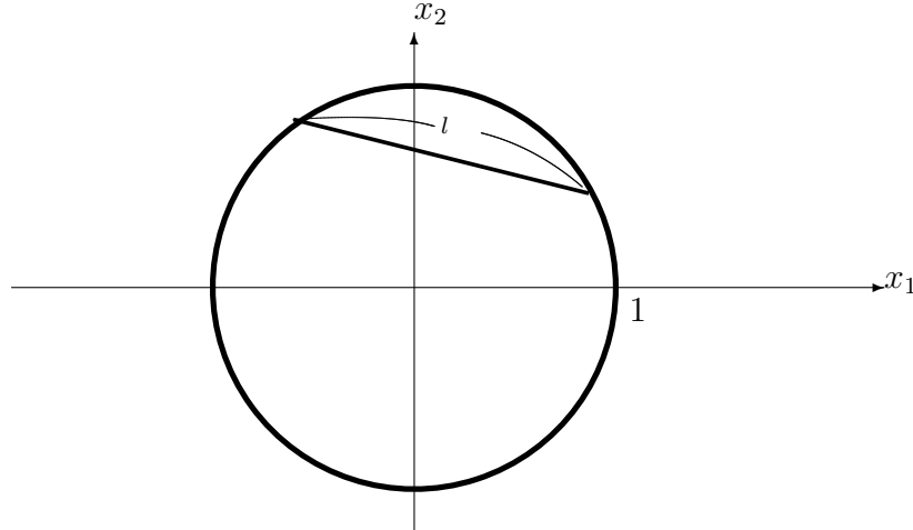
Figure 9.8: Bertrand's paradox
