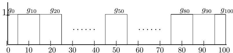
Figure 2.5: Round observable
