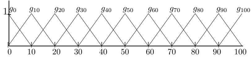
Figure 2.7: Triangle observable
