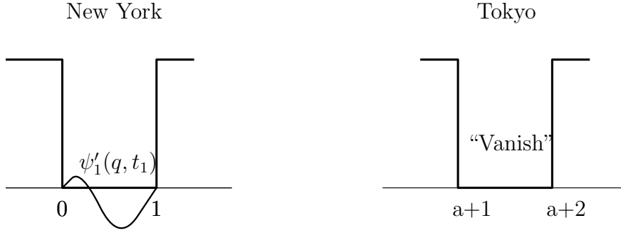
Figure 11.1(4) (The wave function after measurement)
