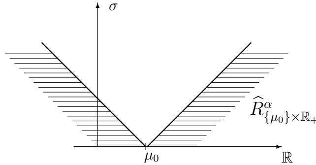
Figure 6.4: Rejection region \hat{R}_{\{\mu_0\}}^{\alpha} (which depends on \sigma )
